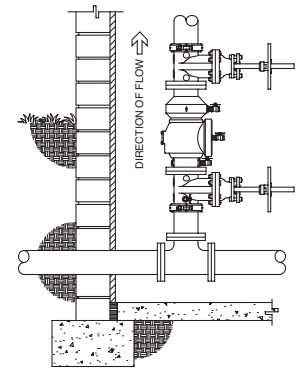
VERTICAL INSTALLATION (350OSYG)
