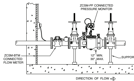
INDOOR INSTALLATION
