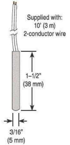
QH521 Remote Sensor
