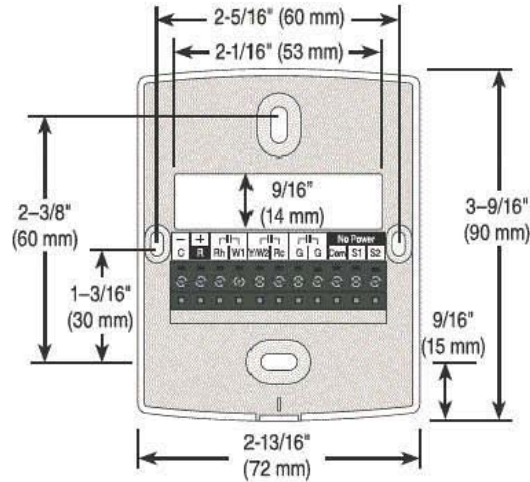
QH521 Mounting Base
