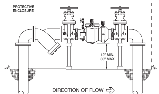
OUTDOOR INSTALLATION MODEL 350AFSC
