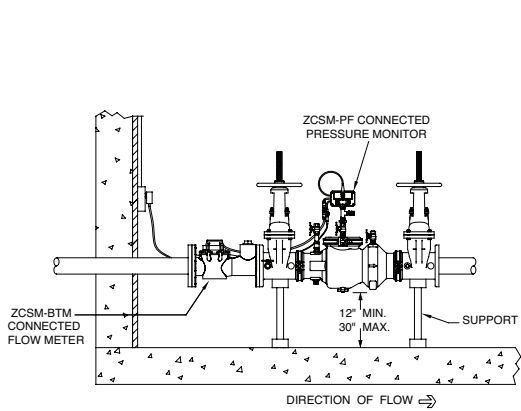
INDOOR INSTALLATION
