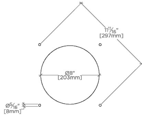
CUTOUT VIEW
