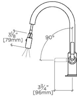
SPRAY AND HANDLE OPERATION
