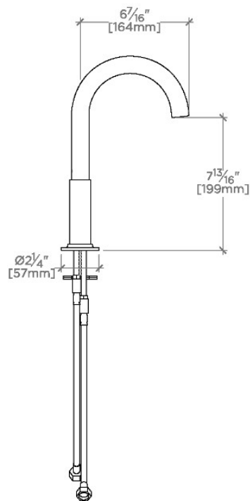
SIDE VIEW SCALE: 1 1/2"=1'-0"
