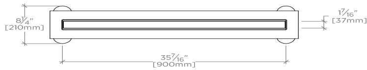
TOP VIEW
