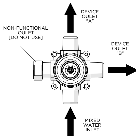
[GUDV2P SHOWN]
