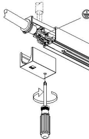
Fig 4b: Live End Connector Feed Options
