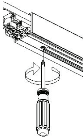
Fig 4a: Live End Connector Track Engagement
