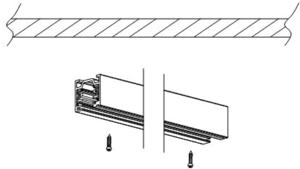
Fig 1: Surface Mount
