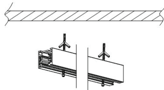
Fig 2: Toggle Bolt Mount
