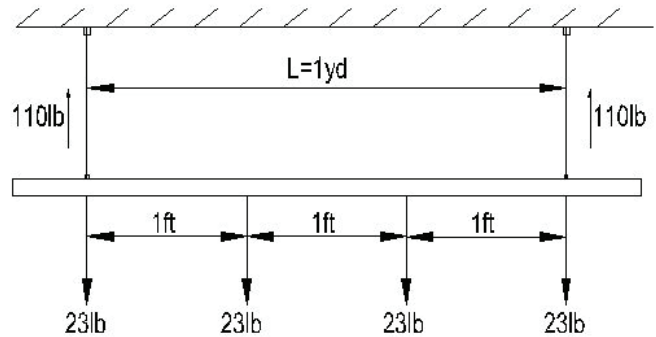
FIG 7A: MAXIMUM LOAD - 1
