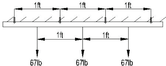
FIG 7C: MAXIMUM LOAD - 3
