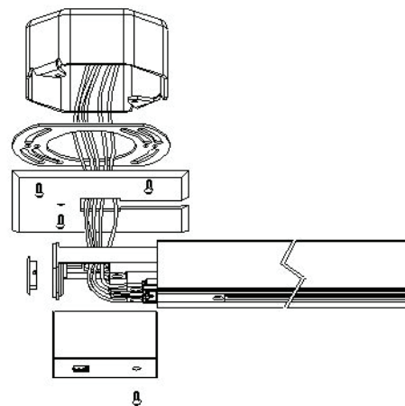
Fig 4b: Live End Connector Feed Options
