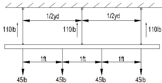
FIG 7B: MAXIMUM LOAD - 2
