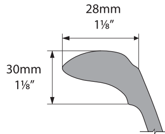
Rim Detail
