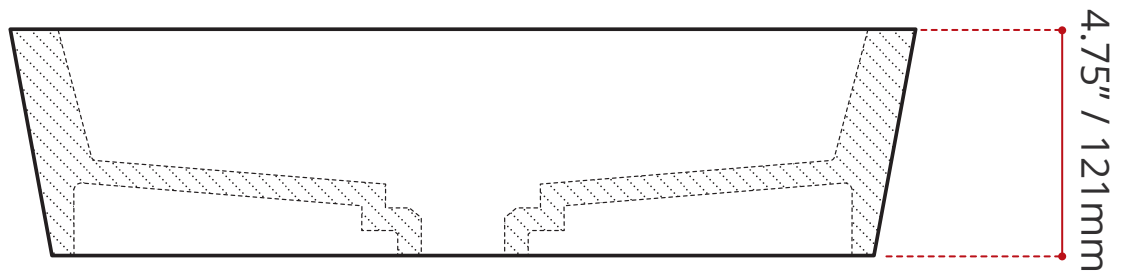
Vessel - Drain portion Cutting Required
