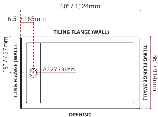
SSTLD6036L1 (LEFT HAND DRAIN LOCATION)
