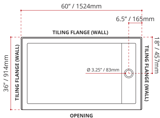
SSTLD6036R1 (RIGHT HAND DRAIN LOCATION)
