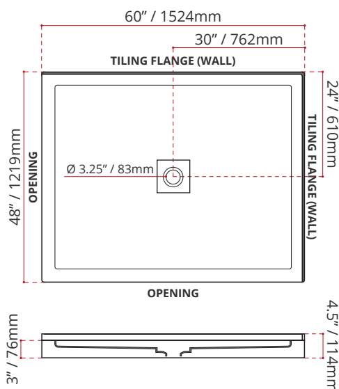
SDTSD6048L1 (LEFT HAND THRESHOLD OPENING)
