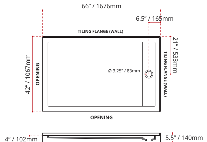
SDTLD6642R1 (RIGHT HAND DRAIN LOCATION) (LEFT HAND THRESHOLD / OPENING)
