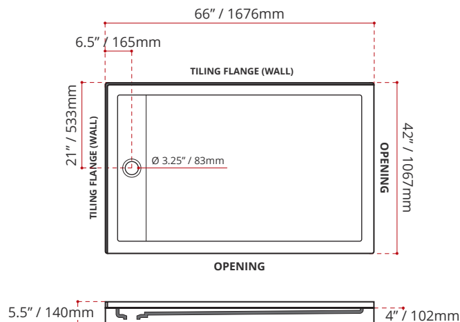
SDTLD6642L1 (LEFT HAND DRAIN LOCATION) (RIGHT HAND THRESHOLD / OPENING)
