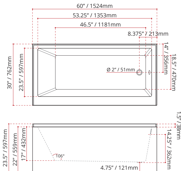
MODEL NUMBER : 2291 (RIGHT HAND DRAIN LOCATION)
