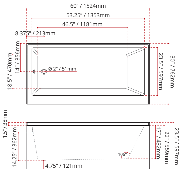
MODEL NUMBER : 2281 (LEFT HAND DRAIN LOCATION)
