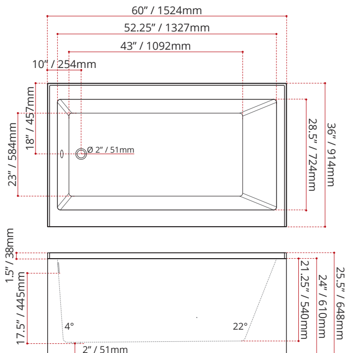
MODEL NUMBER : 2351 (LEFT HAND DRAIN LOCATION)
