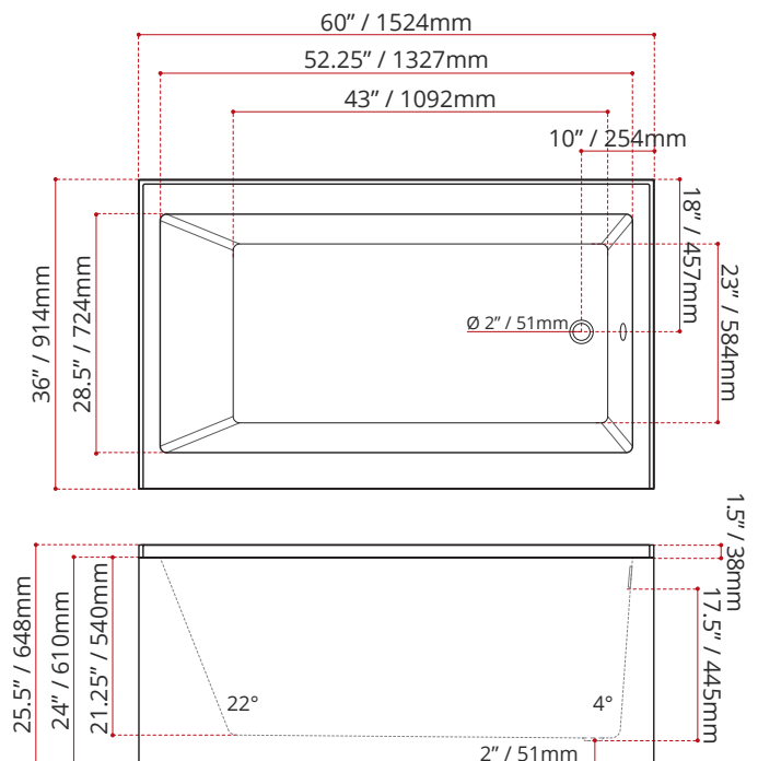
MODEL NUMBER : 2361 (RIGHT HAND DRAIN LOCATION)
