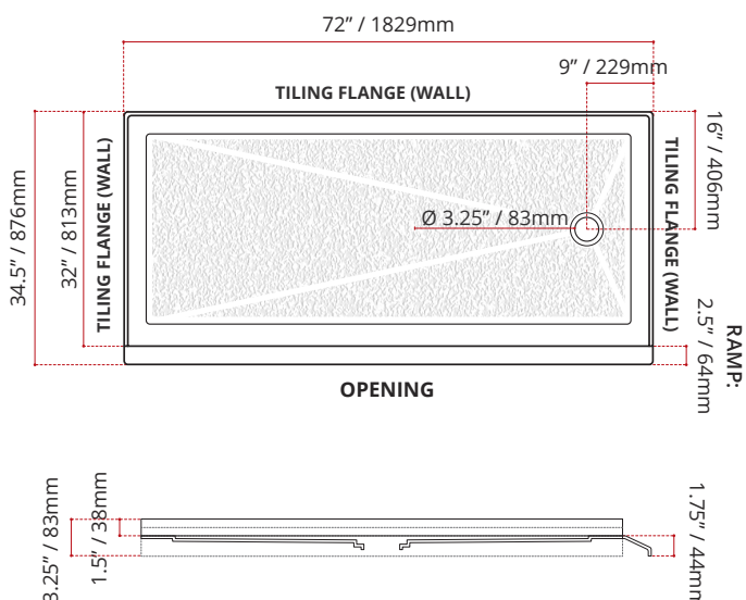
BSSTOD7232R1 (RIGHT HAND DRAIN LOCATION)
