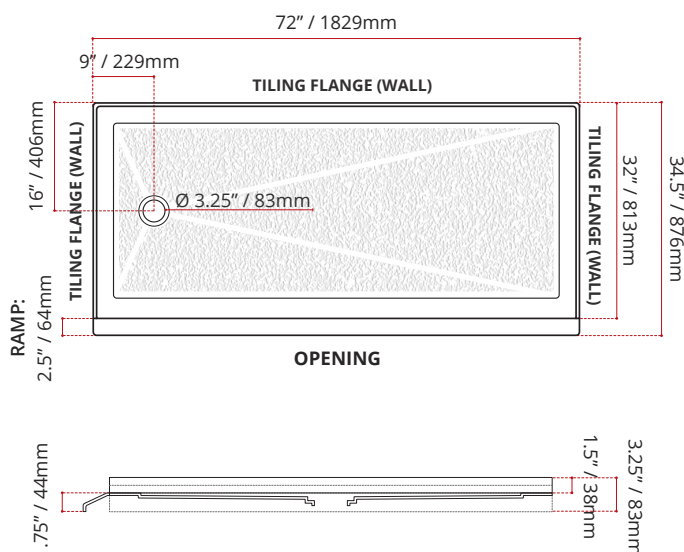
BSSTOD7232L1 (LEFT HAND DRAIN LOCATION)
