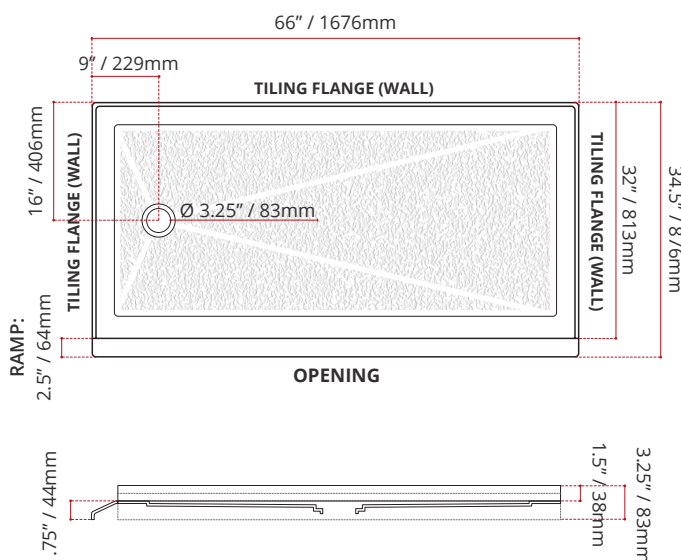
BSSTOD6632L1 (LEFT HAND DRAIN LOCATION)
