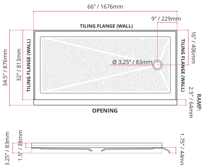
BSSTOD6632R1 (RIGHT HAND DRAIN LOCATION)
