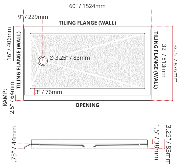
BSSTOD6032L1 (LEFT HAND DRAIN LOCATION)
