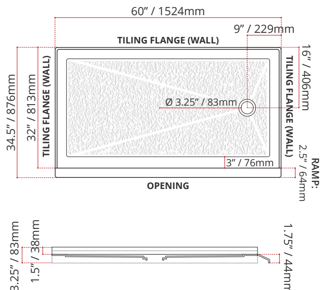
BSSTOD6032R1 (RIGHT HAND DRAIN LOCATION)
