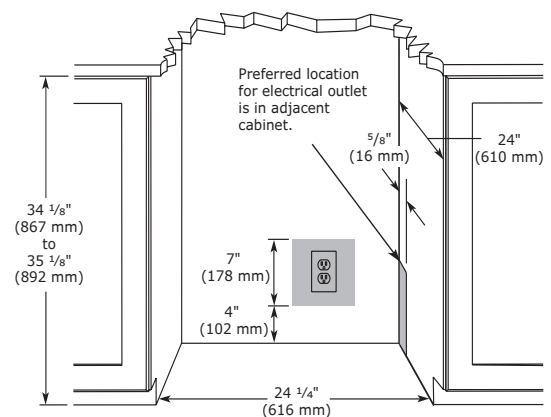
Cabinet Cut-Out
