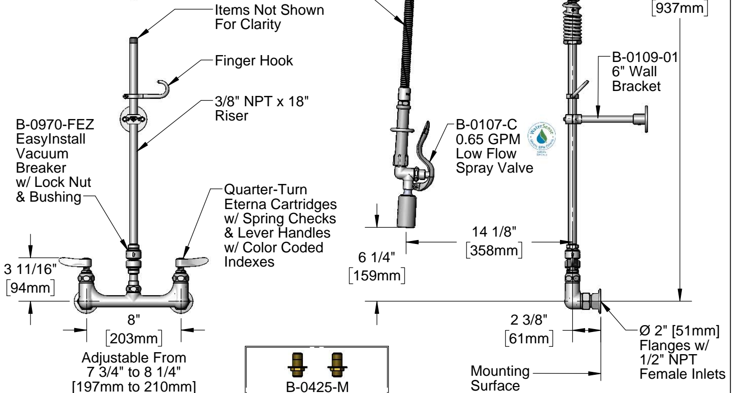
44" Flexible Stainless Steel Hose w/ Spring & Spray Valve
