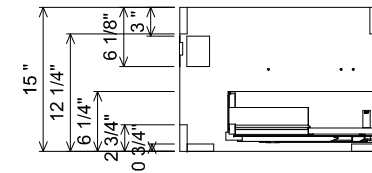
AT SINK CENTER SECTION
