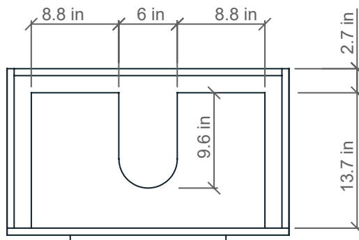
TOP - CABINET ONLY
