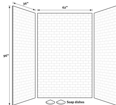
Designed to fit base areas 36" deep or smaller x 62" wide x 96" high or smaller (914 mm x 1575 mm x 2438 mm)
