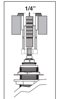
20 Point 3/4" Rough Valve Part # 18.30.xxx
