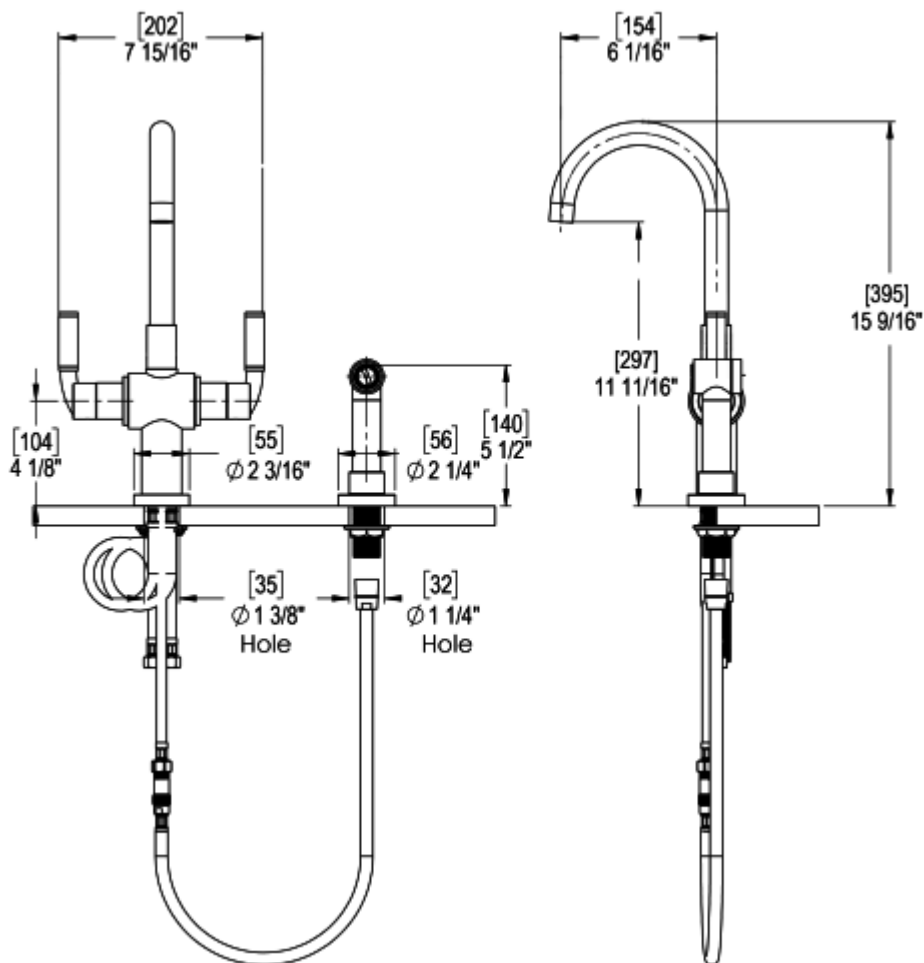
Two Handle Single Hole Bar Faucet with Hand Spray
