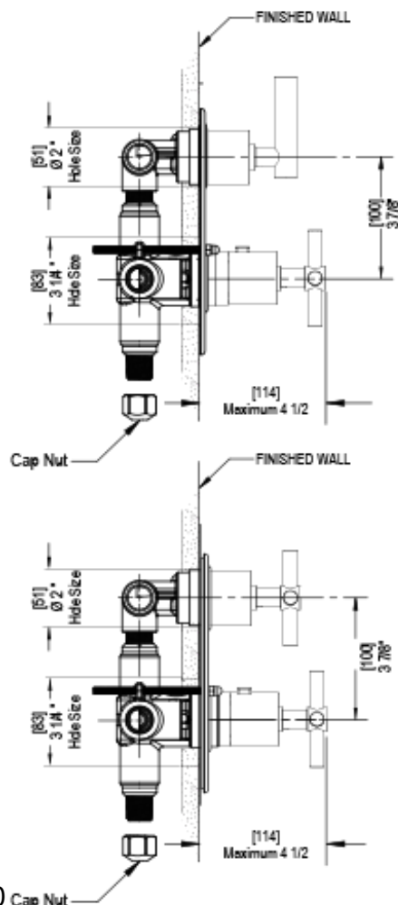
TEMPERATURE CONTROL VALVE WITH STOPS &amp; TWO WAY DIVERTER WITH SHUT-OFF TRIM ONLY
