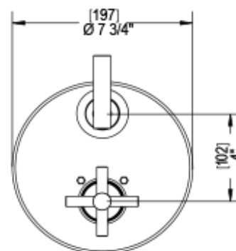
TEMPERATURE CONTROL VALVE WITH STOPS &amp; VOLUME CONTROL
