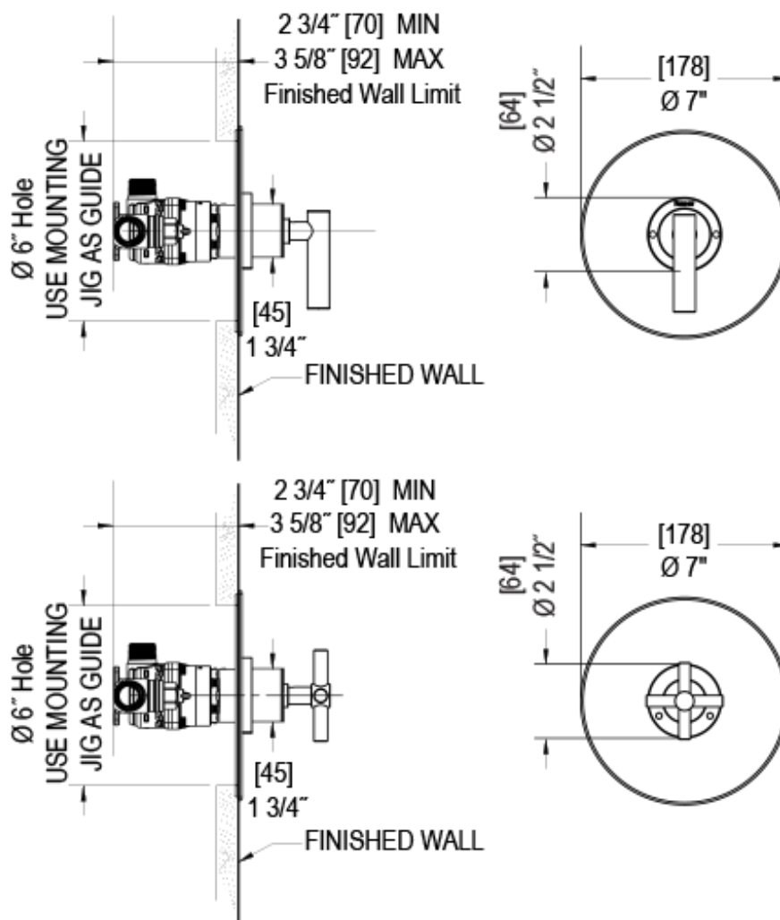
PRESSURE BALANCE SHOWER VALVE WITH STOPS
