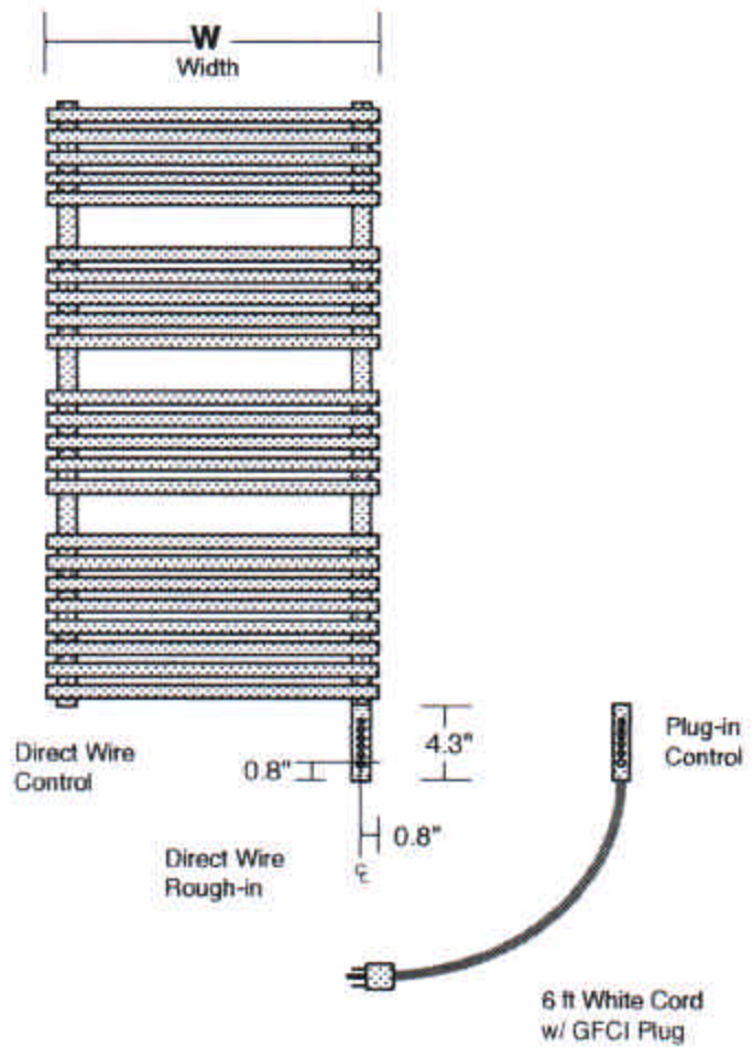
Front View Dimensions
