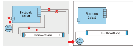
Fig:3 - Retrofit with One Lamp
