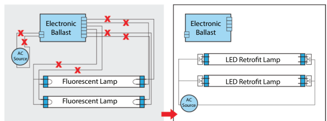
Fig:3 - Retrofit with Two Lamps
