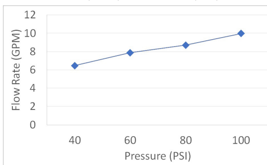
4MT840 Flow Rate (GPM) Vs Pressure (PSI) For Tub Port*
