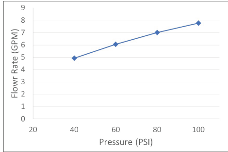
V-2407B Flow Rate (GPM) Vs Pressure (PSI) For Tub Port*
