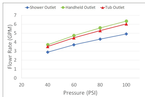
V-2500B Flow Rate (GPM) Vs Pressure (PSI) For Tub Port*
