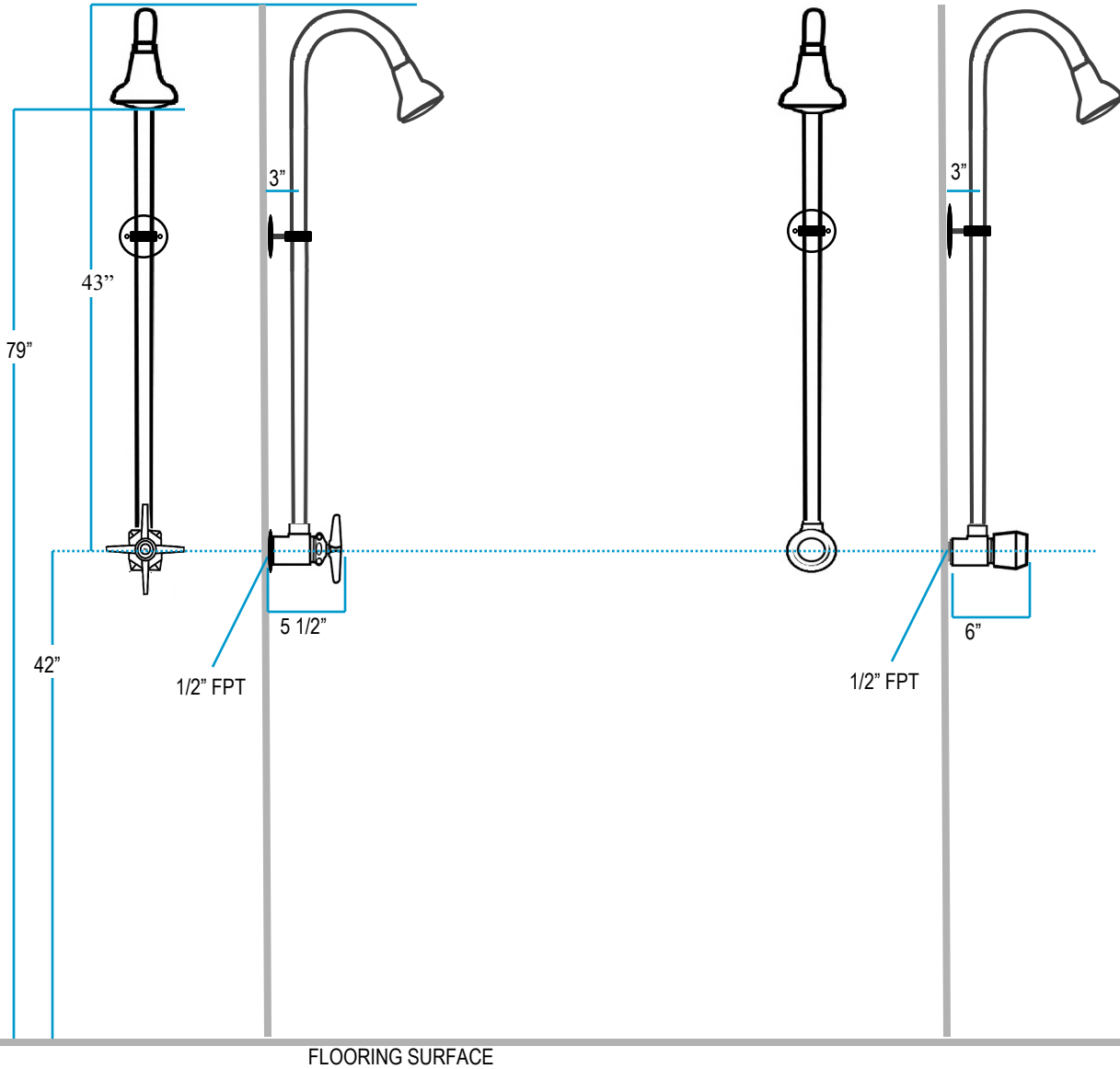
WM-442-CHV FRONT VIEW
