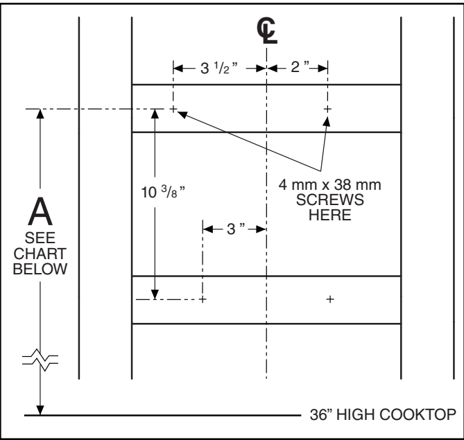
Desired Hood Distance (Above 36" High Cooktop)
