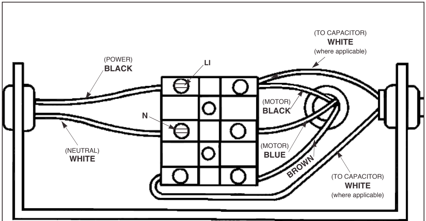
WIRING CONNECTIONS
