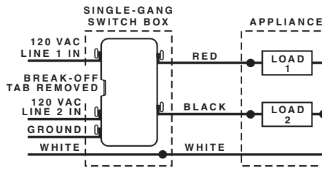
Figure #3 3 ROCKER SWITCH
