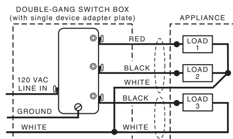
Figure #3 3 ROCKER SWITCH
