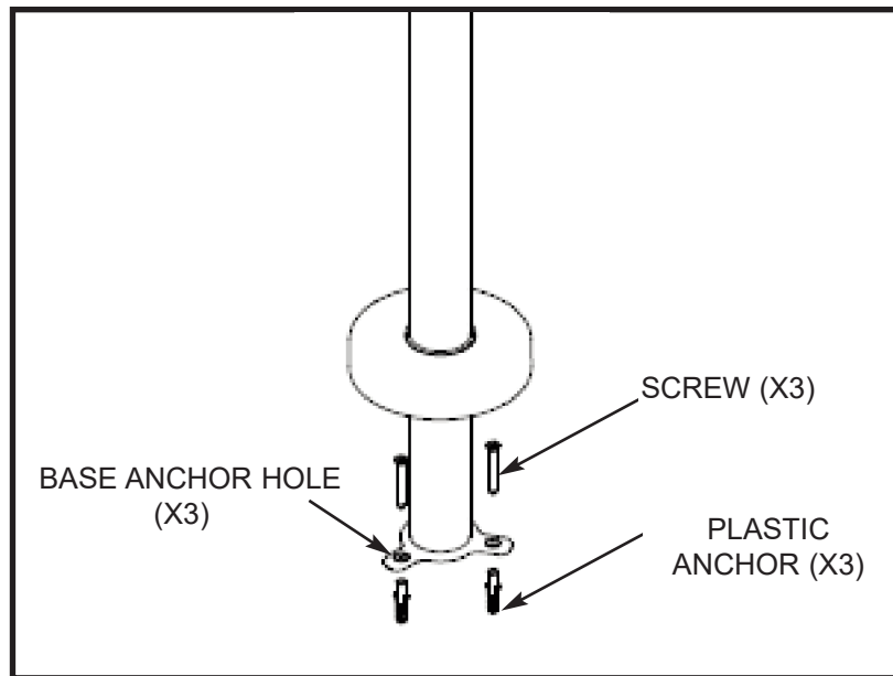
Figure 6 Securing the Tub Filler to the floor.
