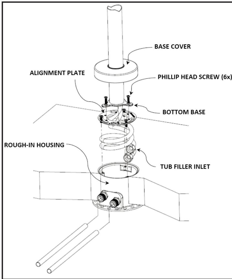
Figure 5 Connecting Tub Filler to the Rough-in Kit 1-339
