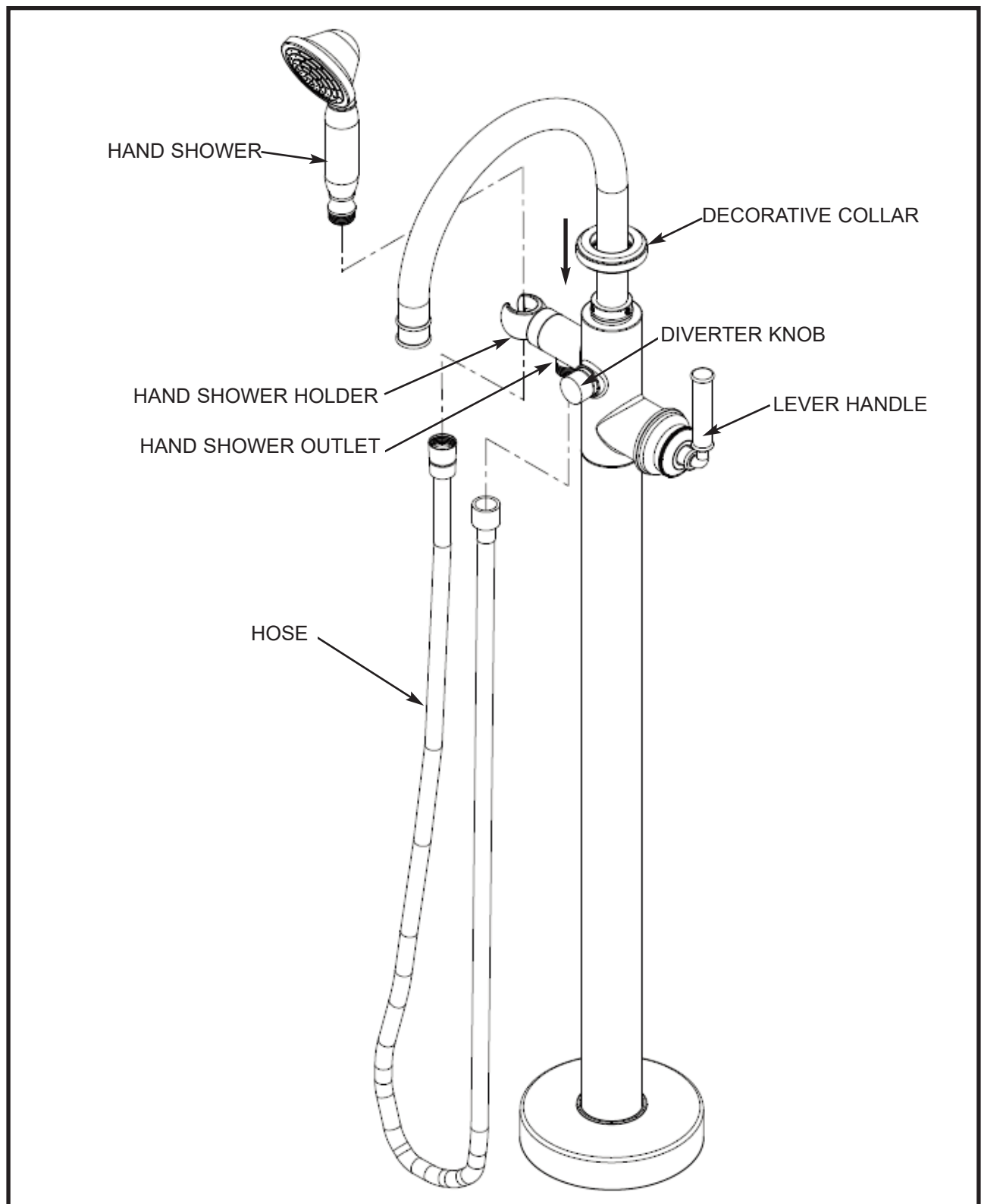
Figure 8 Install the Hose to the Hand Shower and Tub Filler
