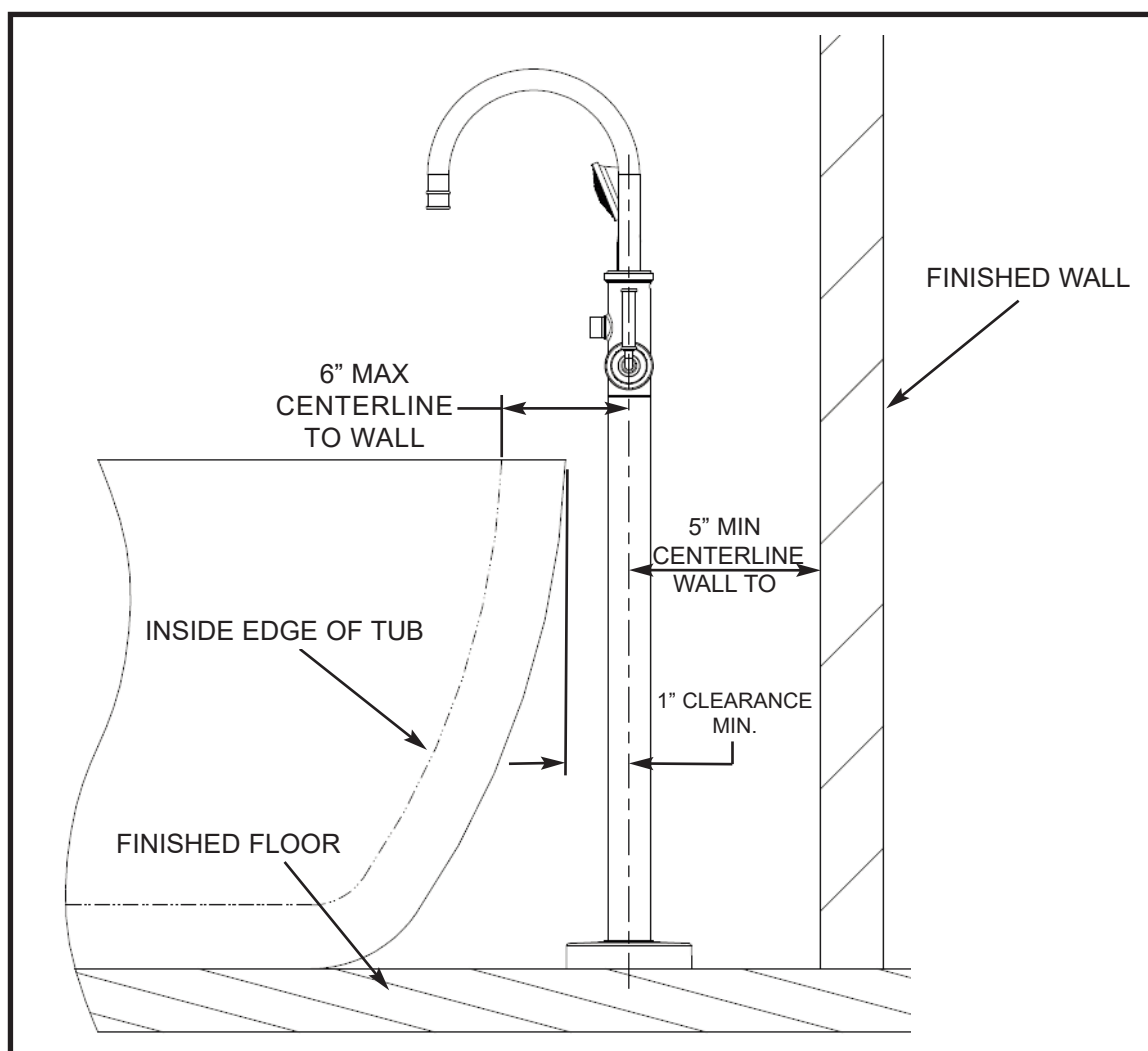
Figure 1 Installation Clearances
