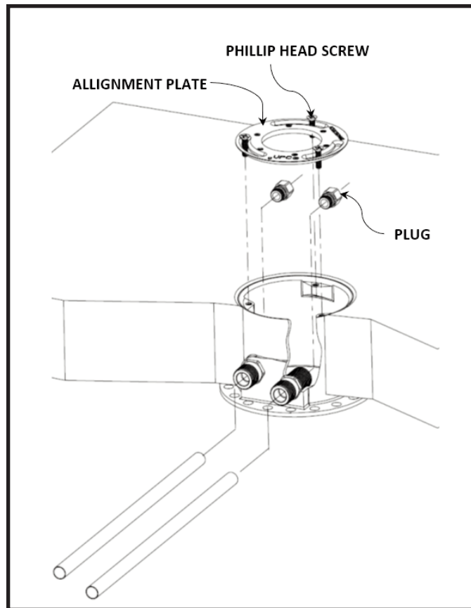
Figure 4 Brasstech Rough-in Kit 1-339
