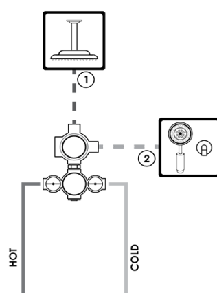
1-745 Thermostatic Valve
