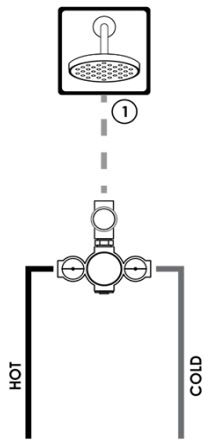
1-741 Thermostatic Valve
