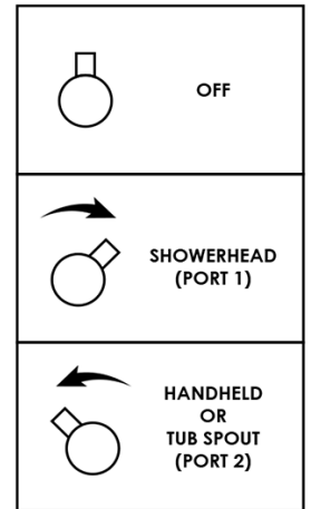
1-742 Thermostatic Valve
