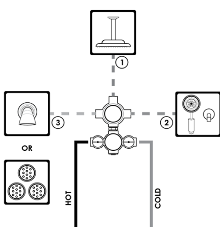
1-743 Thermostatic Valve
