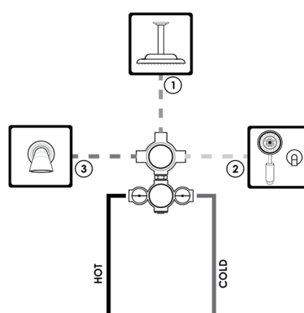
1-744 Thermostatic Valve
