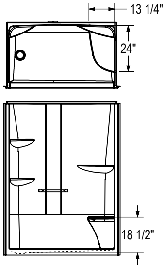
SEAT (Left drain shown)
