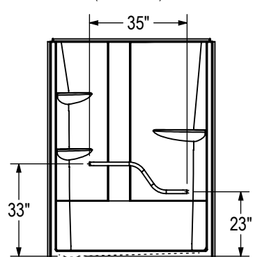
OPTION 20217 (Left Shown)
