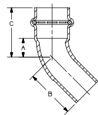
PST45 45° Elbow Ftg x P – Wrot
