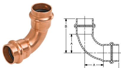
PL90 90° Elbow P x P – Wrot
