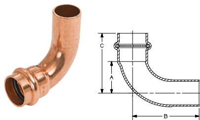
PST90 90° Elbow Ft g x P – Wrot
