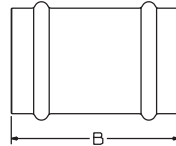
PCPLS (No Stop) Repair Coupling P x P – Wrot
