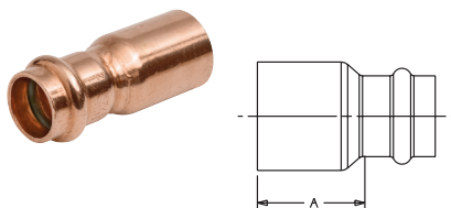
PSTRC Fitting Reducer Ft g x P – Wrot
