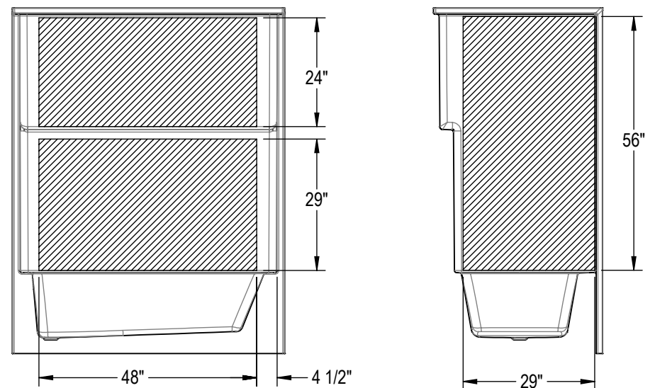
Full Wall Reinforcement Option
