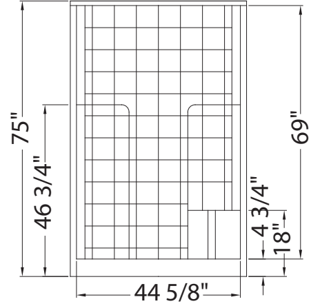
Right seat
