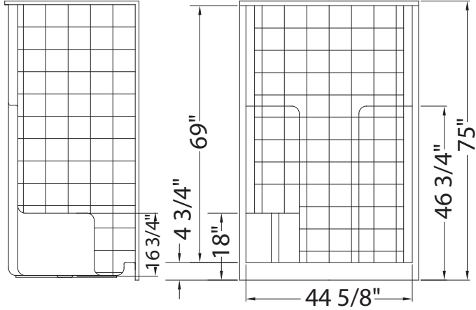
Left seat
