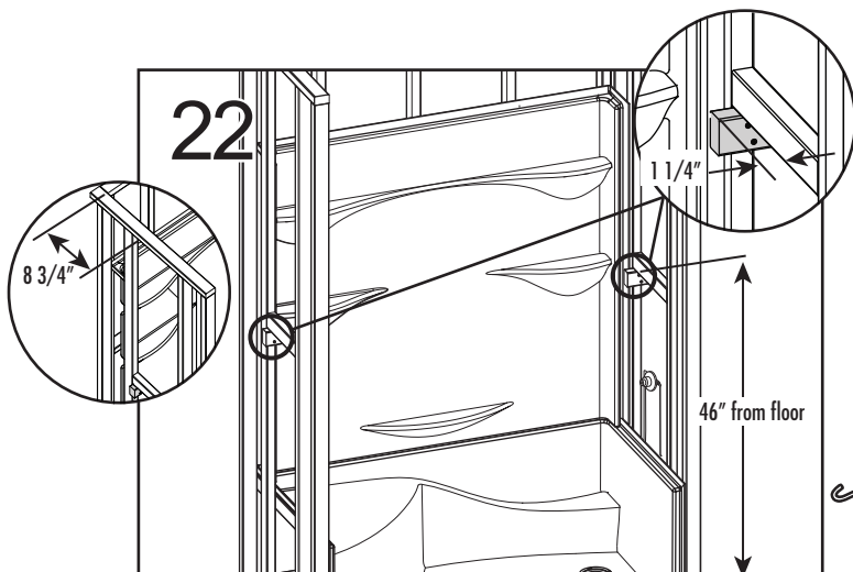
Fix a 2" x 3" x 3 1/2" wood block approximately at 46" from the floor, protruding 1 1/4" to the inside of the shower alcove. The stud supporting the block has to be placed 8 3/4" from the back wall studs.
