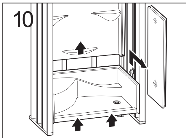
Remove back wall, side wall and base.
