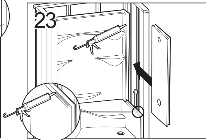
Apply silicone along the inside edge horizontally and vertically. Lay the side wall in position.
