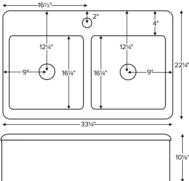
Front view with apron
