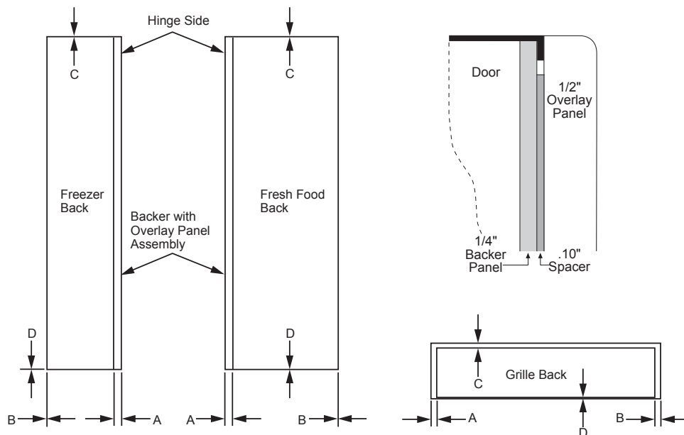
PANEL DIMENSIONS
