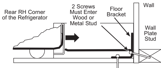
Figure 3 – Attachment to Wall and Floor
