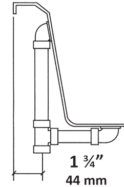
PLUMBING ROUGH-IN
