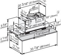
DAS8930, drawing – US
